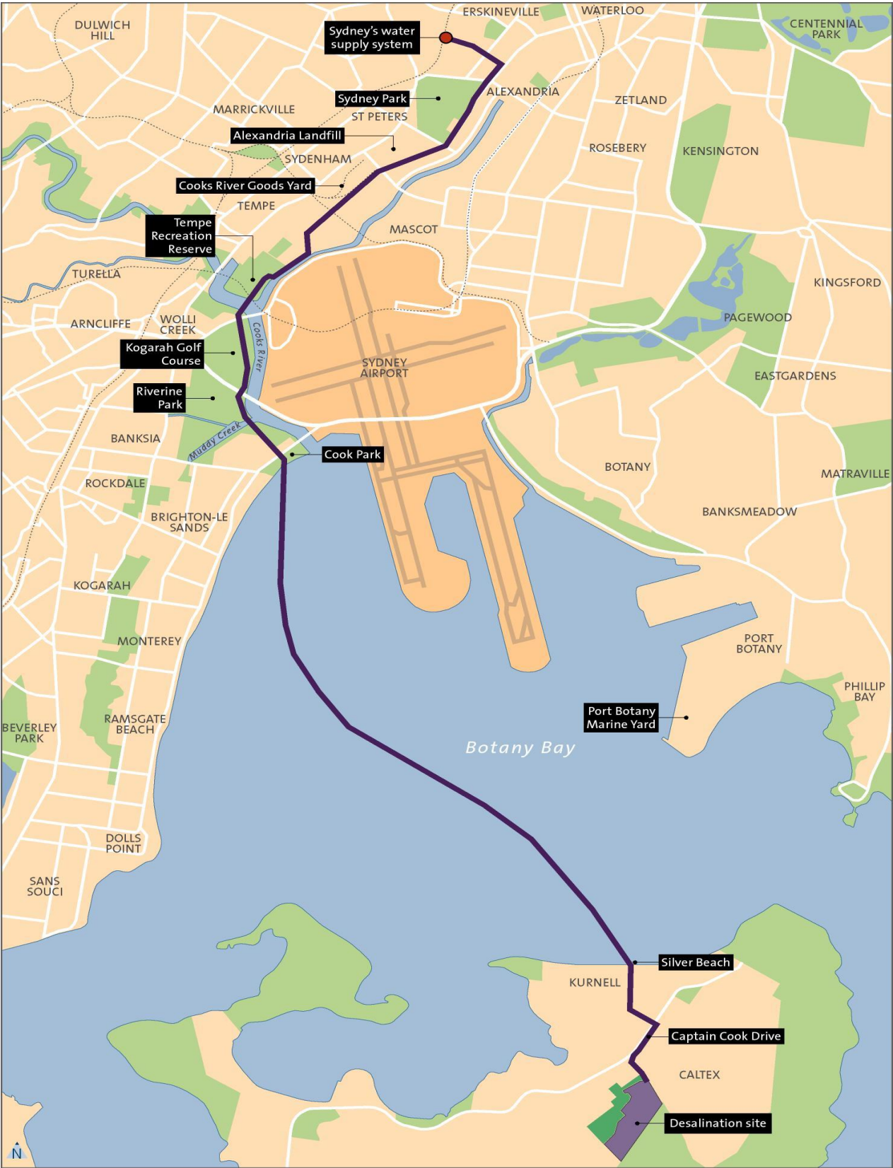
Figure 2.1: Schematic of the Plant and delivery Pipeline to Erskineville
