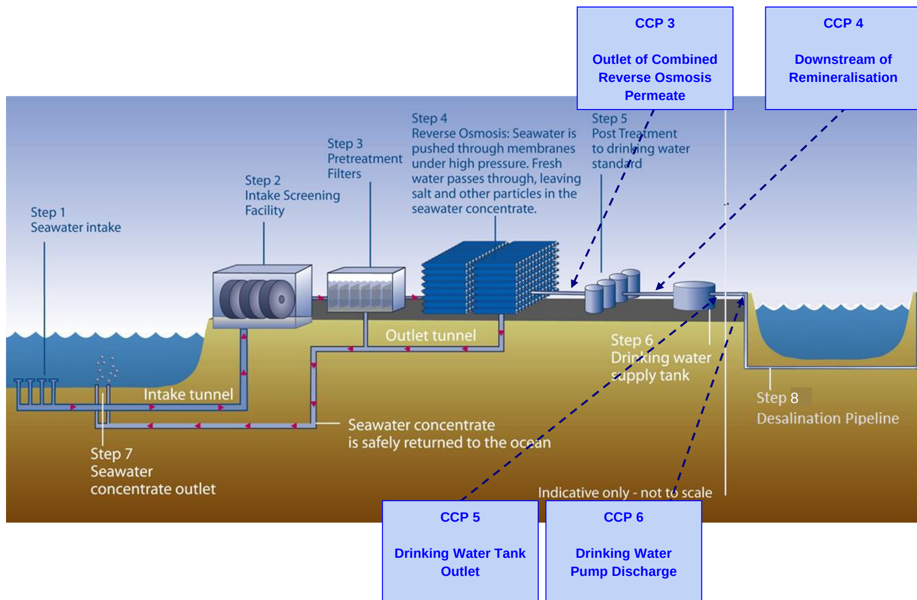
Figure 2.2: Key steps of the desalination plant process including critical control points (CCPs)
